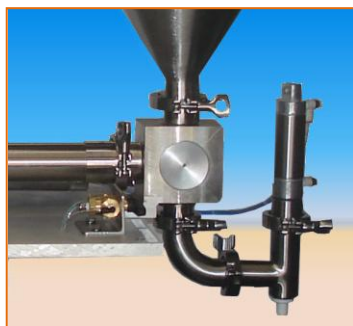
Positive cut-off filling nozzle
